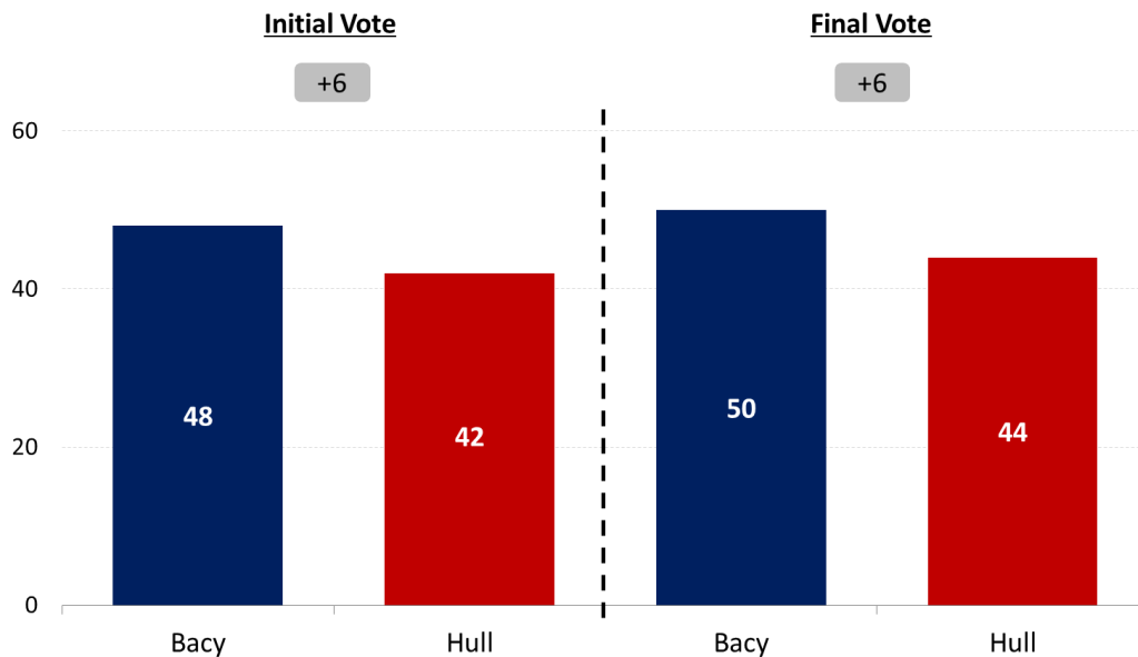
Figure 1: Vote Progression
